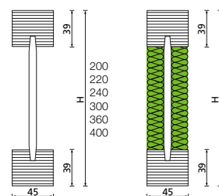
STEICOjoist SJ LVL 45
