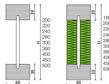
STEICOjoist SJ LVL 60
