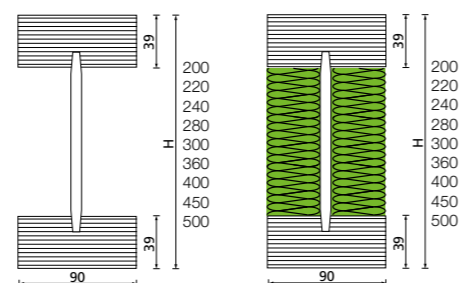
STEICOjoist SJ LVL 90
